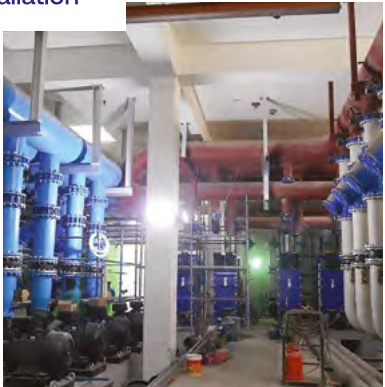
Piping Layout Post-Installation
